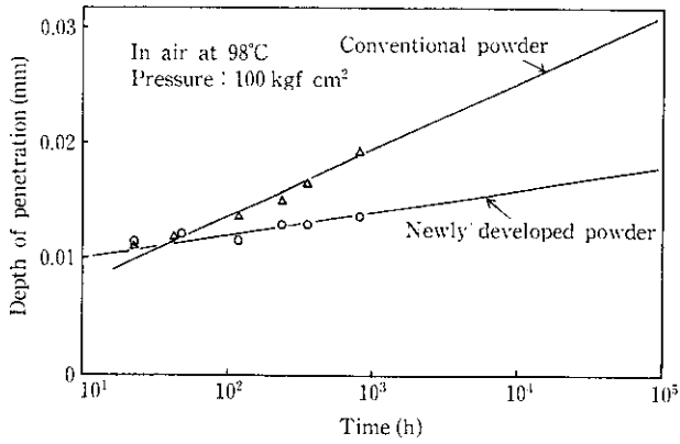
Fig. 2. Time dependence of the depth of penetration of the epoxy resin into the steel pipe.
