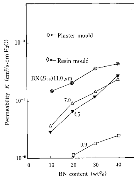
Fig. 4 Effects of BN content and grain size of BN powder on the permeability of Si 3 N 4 -BN ceramics
