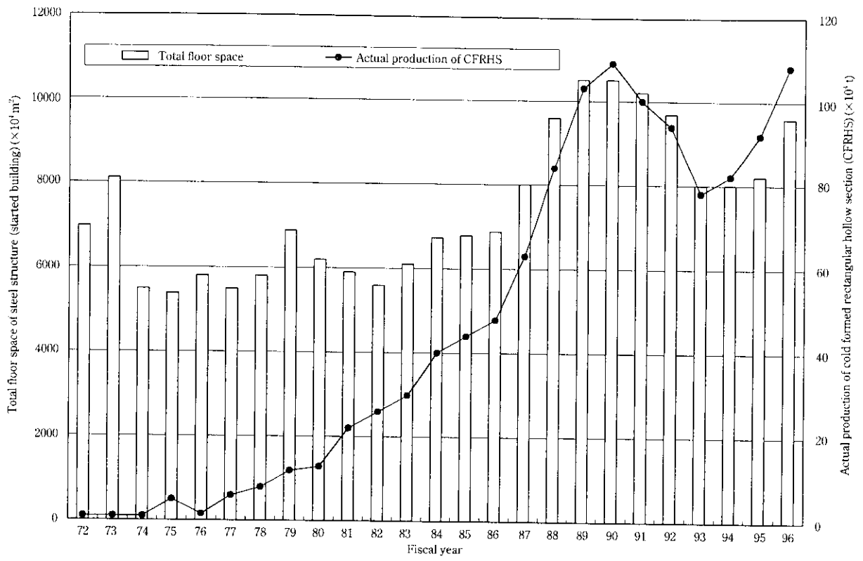
Fig. 2 Change of actual production of column and total floor space
