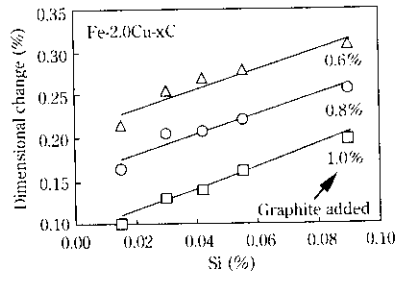
Fig. 3 Effect of Si content in iron powder and added graphite
