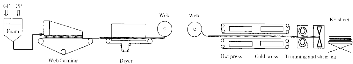
Fig. 1 Manufacturing process of KP sheet
